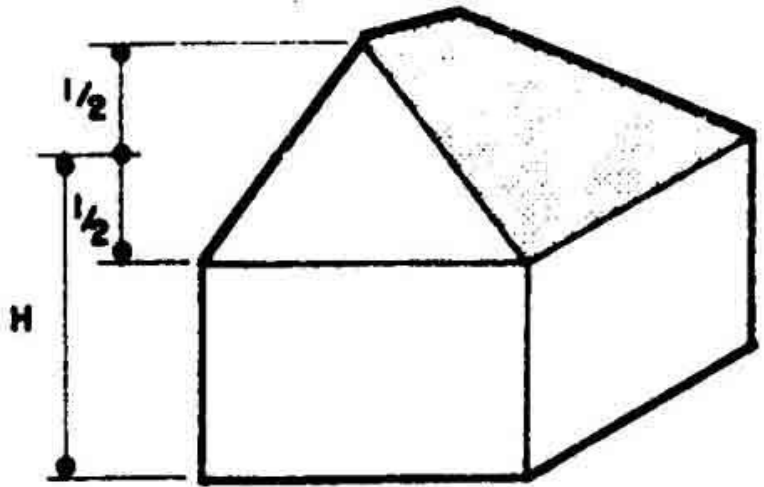
HIP ROOF
